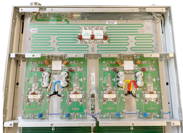
4 X PALLETS com Transistores AMPLION - BLF188XR - 5280W
